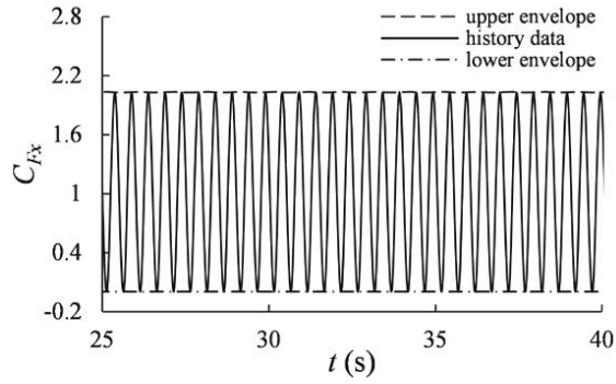
(a) Only rotation motion ( U=1 m/s, \lambda = 2.5 )
