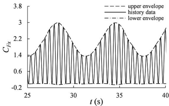
(d) With surging and swaying coupled motion ( U=1 m/s, \lambda = 2.5 , \omega_x = \omega_y = 1 rad/s , A_x = 0.2 m , A_y = 0.2 m )
