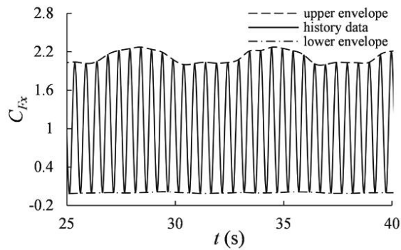
(c) With swaying motion ( U=1 m/s, \lambda = 2.5 , \omega_y = 1 rad/s , A_y = 0.2 m )
