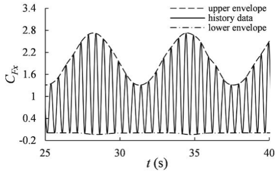
(b) With surging motion ( U=1 m/s, \lambda = 2.5 , \omega_x = 1 rad/s , A_x = 0.2 m )
